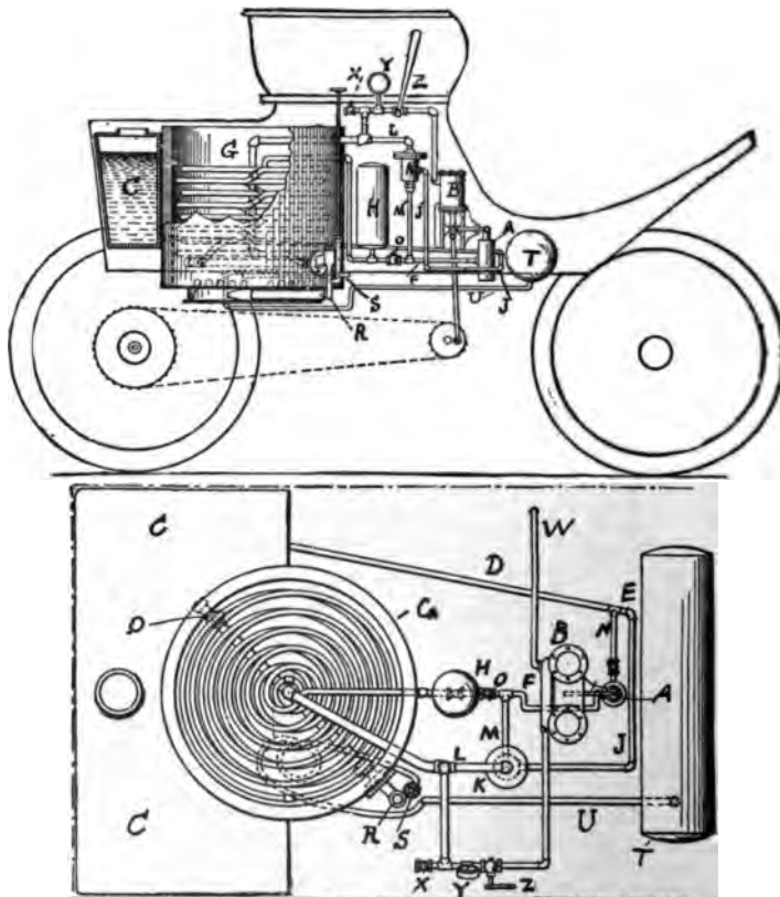
FIG. 358.—Diagram of the Fuel and Water Feed System of the White Steam Carriage. A is the water pump operated from the crosshead of the engine. B, C is the water tank; D, a pipe leading to the pump, and branching off at E, as shown, into J and N. F is the boiler feed pipe leading through the check valve, O, and the air chamber, H. K is the automatic by-pass regulator; L, a pipe leading steam from the generator, G, and allowing the water to circulate through F, M, K, J, E, N, A, whenever steam pressure rises high. X, the pop valve; Y, the gauge; Z, the throttle; T, the fuel tank; U, the fuel feed pipe; Q, R, S, the fuel regulating and vaporizing system explained later.
